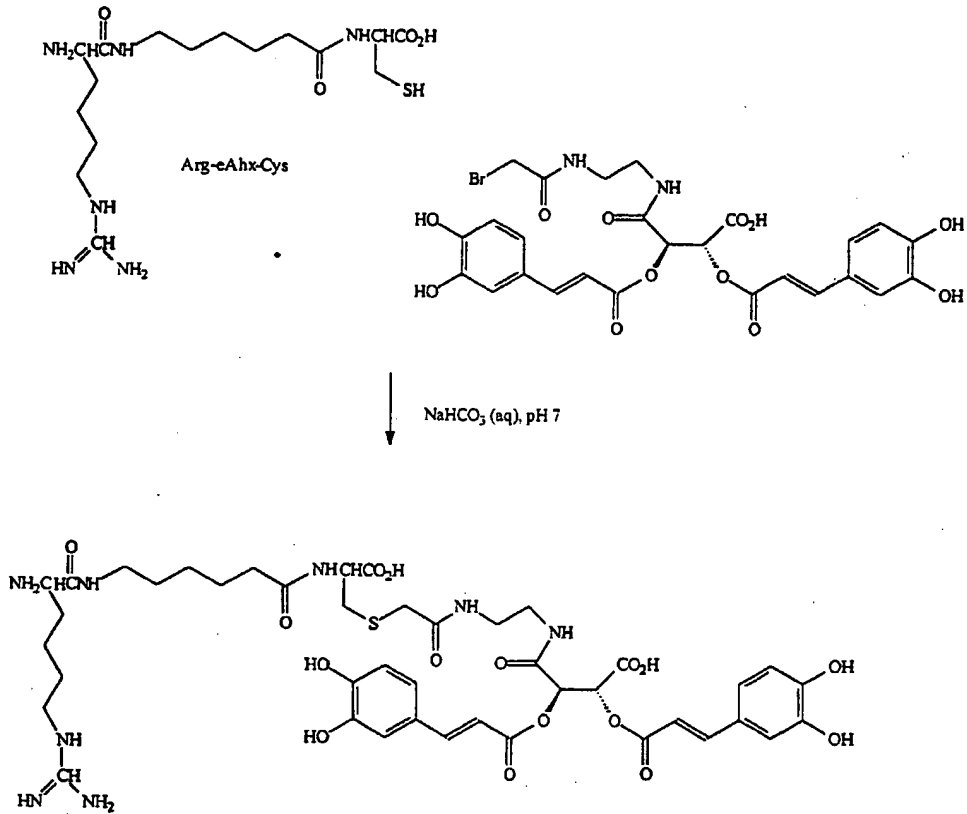
Scheme 4 Conjugation of recognition/linker to bromoacetylated L-chicoric acid
